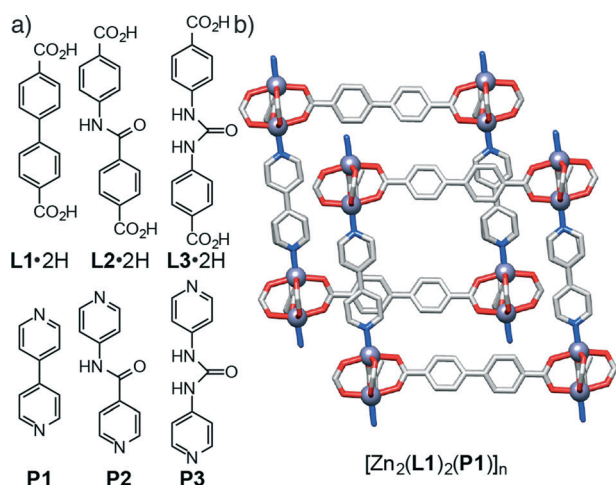
Fig. 1 a) Structures of the diacid ligands (L1-2H–L3-2H) and di-pyridinyl pillars (P1–P3) examined in this study. b) Portion of the solid-state structure of [\text{Zn}_2(\text{L1})_2(\text{P1})]_n , the basic framework upon which the work is based. Redrawn from CCDC deposition FEFCUQ with hydrogen atoms and disorder omitted for clarity.
