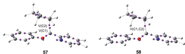
Fig. 14 Selected structures 57 and 58 of the IRC associated with the formation of the first C–C single bond in I-DA reactions between oxonium cation 54 and cyclopentene 55 .
