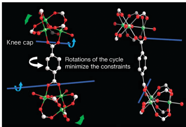
Fig. 11 Depiction of the hinge in MIL-88 around which the rotation that induces the pore swelling occurs. (Reprinted with permission. 133 Copyright 2007 American Association for the Advancement of Science.)
