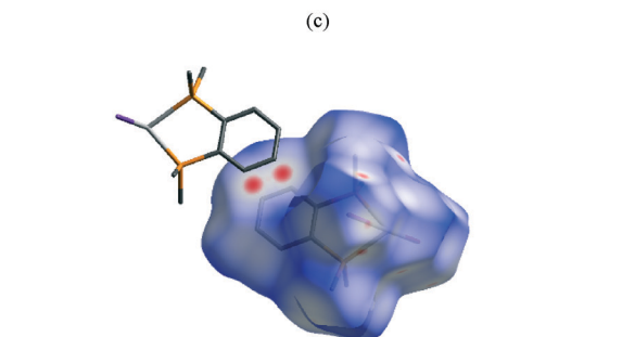
Fig. 9 View of a section of the aromatic...aromatic interface in 1 at ambient pressure (a), illustrating the edge-to-face arrangement of the benzene rings (angle between the adjacent rings ranges from 81° to 73° at ambient and 48 kbar respectively); corresponding Hirshfeld surface for 1 (b) with normalised contact distance, d_{\text{norm}} , mapped onto the surface; the equivalent interface in 3 (c), showing the offset-parallel arrangement of the rings; corresponding Hirshfeld plot for 3 (d). Red regions correspond to negative values of d_{\text{norm}} where contacts are closer than the van der Waals separation, blue positive and longer than vdW separation and white around the van der Waals separation geometric details are in Table S2.†
