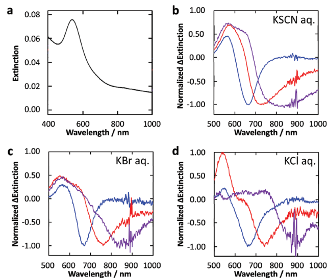
Fig. 2 (a) Extinction spectrum of Au NPs deposited photocatalytically on the TiO 2 film. (b–d) Normalized difference extinction spectra of Au NPs on TiO 2 after 600–700 nm (blue), 700–800 nm (red) and 800–1000 nm (purple) light irradiation (10 mW cm -2 , 30 min) in 0.5 M aqueous solution of (b) KSCN, (c) KBr and (d) KCl.
