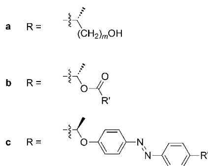
Chart 12 Poly( N -propargylamide)s derived from optically active hydroxycarboxylic acids.
