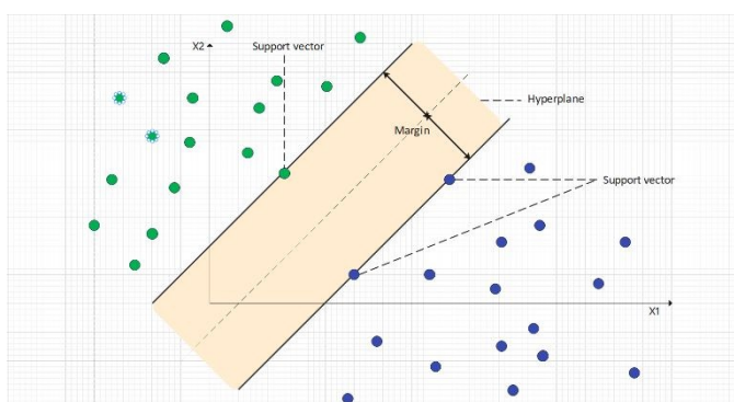
Figure 4 Support vectors and hyperplane in Supporting Vector Machine algorithms.
