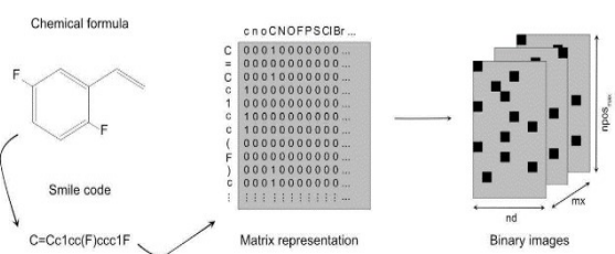
Figure 9 Illustration of how each monomer was transferred into a matrix, then converted into a binary image. Reproduced from ref. 110 with permission from Elsevier, copyright 2020.
