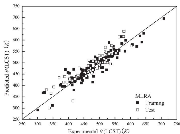
Figure 13 The prediction performance of the MLR model on both training and testing sets. Reproduced from ref. 117 with permission from John Wiley and Sons, copyright 2008.
