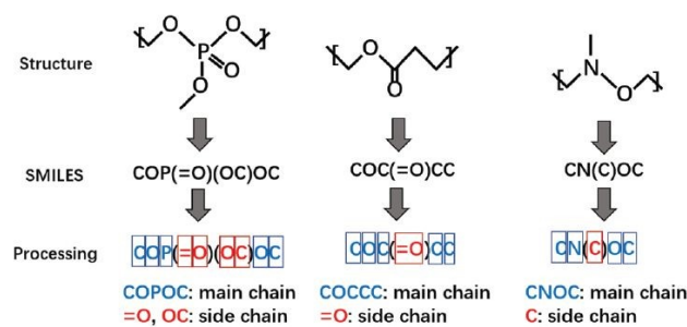
Figure 7 The process of converting polymer structures to SMILES strings and further preparation to generate input descriptors for machine learning models. Reproduced from ref. 109 with permission from the Royal Society of Chemistry, copyright 2021.
