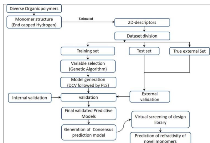
Figure 11 The workflow of the QSPR study about the refractive index of the polymer. Reproduced from ref 113 with permission from the American Chemical Society, copyright 2018.
