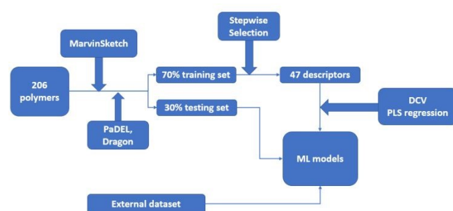
Figure 12 The workflow of the QSPR study about the glass transition temperature prediction with Machine Learning.
