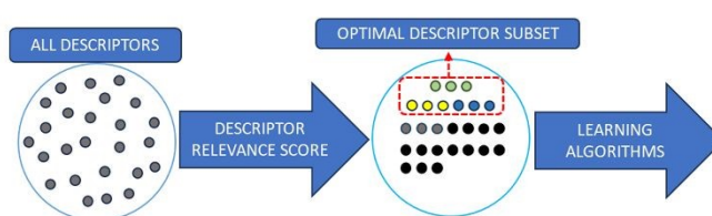
Figure 3 Descriptor Selection Workflow. The relevance score for each descriptor is computed. Based on the score, descriptors are ranked, and an optimal descriptor subset is identified. This subset is then fed into machine learning algorithms.
