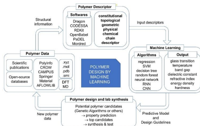
Figure 1 The critical components of polymer design with the aid of machine learning.
