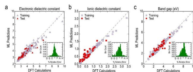
Figure 18 ML prediction and DFT calculation comparison on three properties: electronic dielectric constant, ionic dielectric constant, and band gap. Reproduced from ref. 108 with permission from Nature Publishing Group, copyright 2016.
