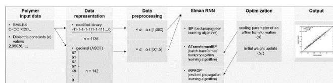
Figure 8 The binary and decimal transformation of SMILES strings. Reproduced from ref. 36 with permission from the American Chemical Society, copyright 2021.
