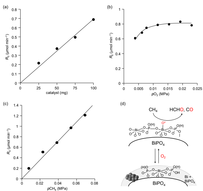
Fig. 6 Effect of (a) catalyst amount and partial pressure of (b) O_2 and (c) CH_4 on reaction rate. Reaction conditions for (a): BiPO_4 -DEG (25–100 mg), CH_4/O_2/N_2 (5/1/7 sccm; total 13 sccm), reaction temperature ( 550\text{ }^\circ\text{C} ). Reaction conditions for (b): BiPO_4 -DEG (100 mg), CH_4/O_2/N_2 (5/0.5–3/7.5–5 sccm; total 13 sccm), reaction temperature ( 550\text{ }^\circ\text{C} ). Reaction conditions for (c): BiPO_4 -DEG (100 mg), CH_4/O_2/N_2 (1–9/1/11–3 sccm; total 13 sccm), reaction temperature ( 550\text{ }^\circ\text{C} ). (d) Proposed reaction mechanism for oxidation of CH_4 with O_2 over BiPO_4 -DEG.
