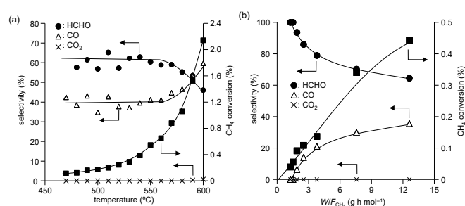
Fig. 4 (a) Product selectivity and CH 4 conversion as function of reaction temperature with O 2 over BiPO 4 -DEG. Reaction conditions: BiPO 4 -DEG (100 mg), CH 4 /O 2 /N 2 (2/2/6 sccm). (b) Effect of W/F_{CH_4} on product selectivity and CH 4 conversion. Reaction conditions: BiPO 4 -DEG (100 mg), CH 4 /O 2 /N 2 (38:8:54 molar ratio; total 7.8–78 sccm), reaction temperature (550 °C).
