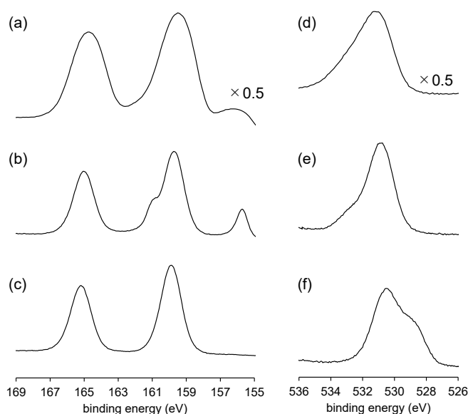
Fig. 7 XPS (a–c) Bi 4f and (d–f) O 1s spectra of BiPO_4 -DEG. (a and d) BiPO_4 -DEG at room temperature under evacuation, (b and e) BiPO_4 -DEG at 550\text{ }^\circ\text{C} under evacuation, and (c and f) BiPO_4 -DEG at 550\text{ }^\circ\text{C} under O_2 (0.1 mbar).
