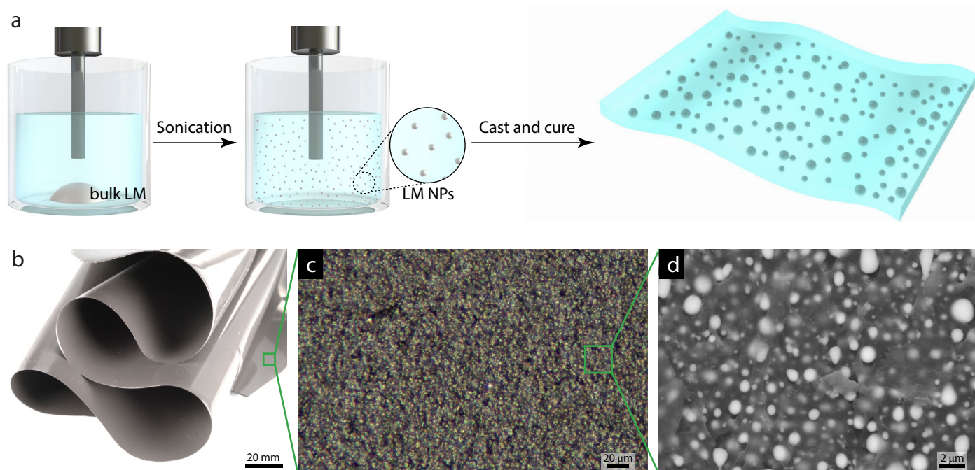
Fig. 1 Liquid metal soft composites. a) Schematics showing the fabrication of LM nanodroplets using probe sonication. b) Photograph showing the soft, flexible nature of the LM composites. c) Optical micrograph and d) SEM image of a composite showing LM microstructure.
