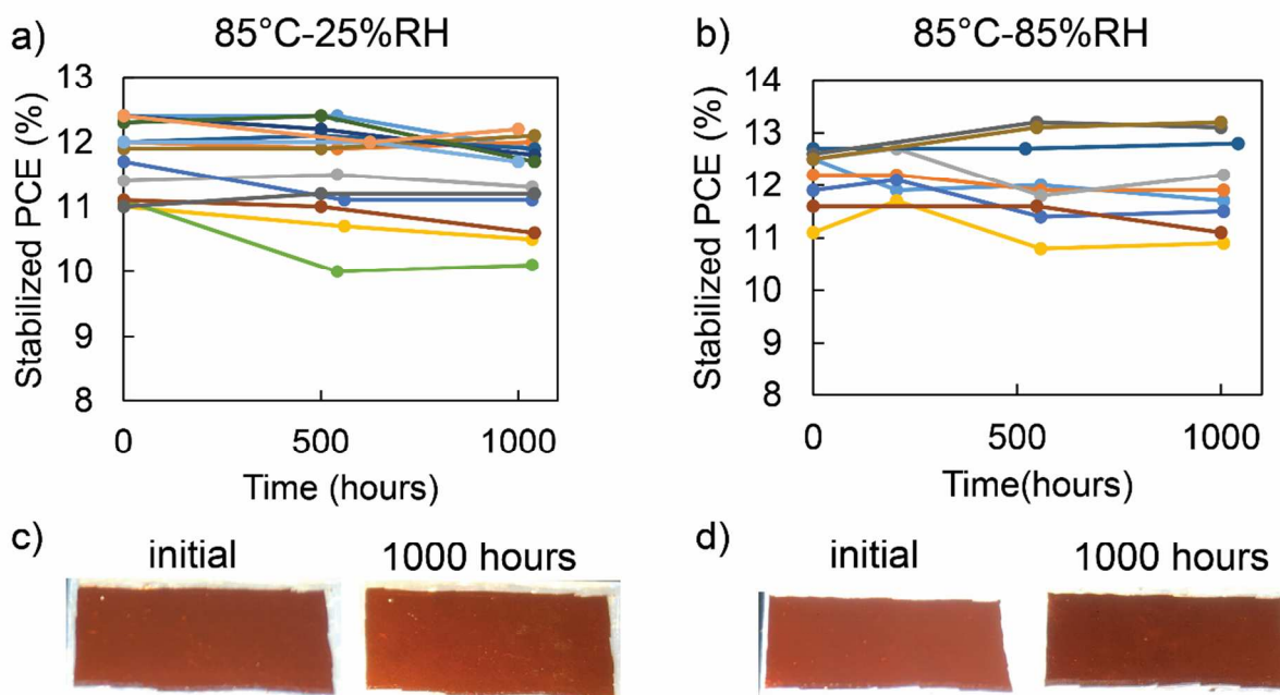
Figure 4: Stabilized maximum power efficiency for 2 nd generation-packaged PSCs with the ENLIGHT polyolefin as they went through a) 85°C-25% RH or “dry heat” and b) 85°C-85%RH or “damp heat”. Representative pictures of the encapsulated solar cells in c) dry heat d) damp heat taken under the solar lamp before and after 1000 hours of aging.
