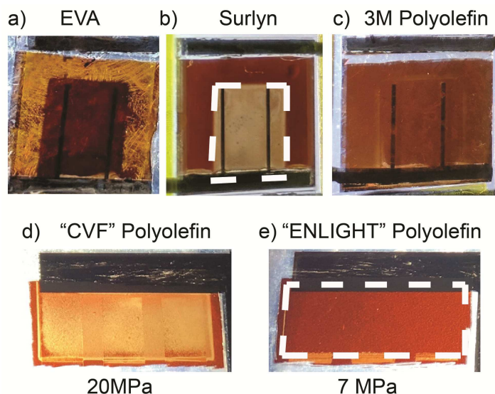
Figure 2: Pictures taken under a solar lamp of the 1 st generation encapsulated PSCs in a) Ethylene Vinyl Acetate (EVA) b) Surlyn c) 3M's Polyolefin after 20 hours at 120°C-100% relative humidity. Another set of pictures taken under the lamp of the 2 nd generation encapsulated PSCs in d) "CVF" Polyolefin with 20 MPa elastic modulus and e) "ENLIGHT" Polyolefin with 7 MPa elastic modulus after 1024 hours aging at 85°C in ambient. The top protective ITOs are outlined in b) and e) as dash rectangles.
