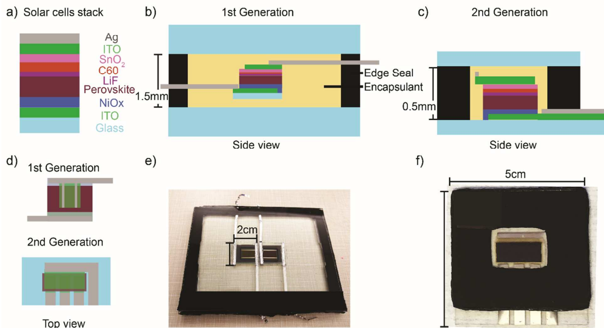
Figure 1: a) PSC stack in this study. Side view of b) 1 st generation c) 2 nd generation package assembly (not to scale). d) Top view of both package generations. Top view image of e) 1 st generation f) 2 nd generation package after lamination.
