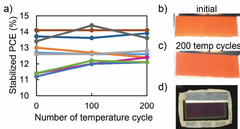
Figure 3: a) Stabilized power conversion efficiency of nine solar cells over 200 temperature cycles between -40°C and 85°C. Representative picture of the ENLIGHT encapsulated PSCs b) initial c) 200 temperature cycles taken under the solar lamp. d) Top view of a representative package after temperature cycling shows no sign of delamination or blistering.
