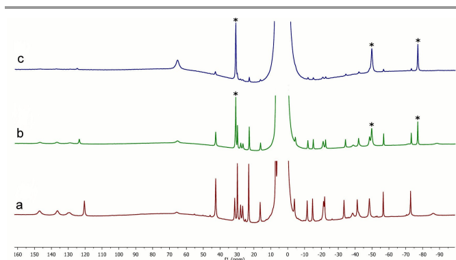
Figure 4. (a) ^1\text{H} NMR spectrum of complex 14b in THF. (b) 14b + 20 \text{BnMgCl} , after 10 min. (c) As above, after 5 h; peaks marked '*' correspond to 'ate' complex 12 .
