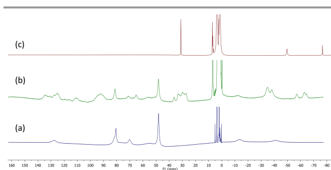
Figure 5. (a) ^1\text{H} NMR spectrum of complex 8 . (b) and (c) Spectra recorded after addition of 2 and 4 equiv. \text{BnMgCl} respectively.
