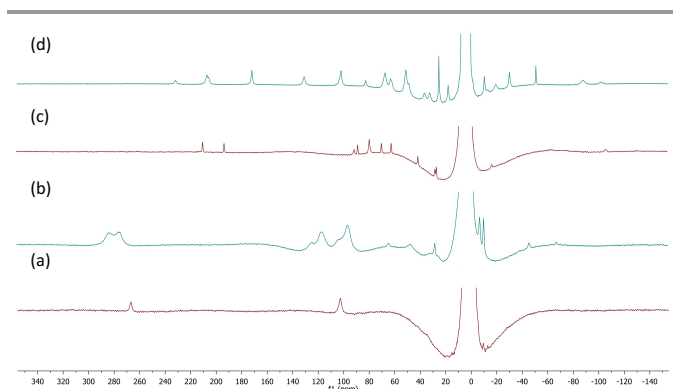
Figure 6. (a) and (c) ^1\text{H} NMR spectra of complexes 9 and 10 respectively (THF, r.t.); (b) and (d) Spectra recorded 10 minutes after addition of 10 equiv. \text{BnMgCl} to 9 and 10 respectively.
