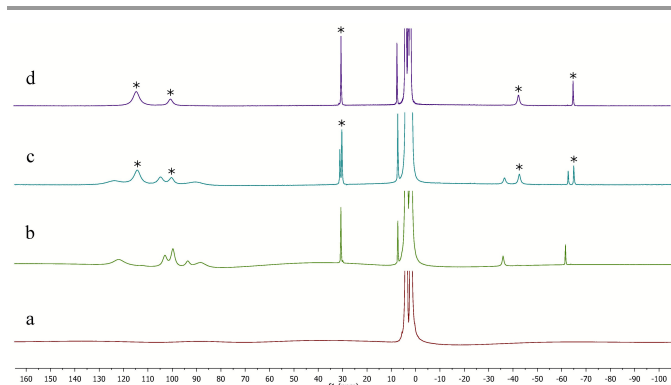
Figure 3. (a) ^1\text{H} NMR spectrum of complex 6 in THF (NMR silent). (b) Part of spectrum of complex 15 , formed in situ from 6 and 1 equiv. \text{BnMgCl}/\text{Fe} (peak at 1067 ppm omitted). (c) and (d) addition of a further 0.5 and 1 equivalent of \text{BnMgCl}/\text{Fe} . Peaks marked '*' correspond to [\text{FeBn}_2(\text{TMEDA})] , ( 14a ).
