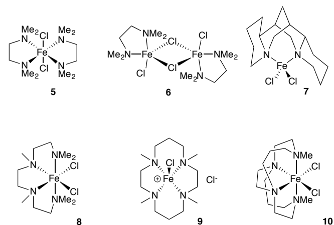
Figure 1. The iron complexes examined.
