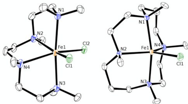
Figure 2. X-ray crystal structures of complexes 8 and 9 . Thermal ellipsoids set at 50% probability; hydrogen atoms, chloride counter-ion of 9 and three molecules of MeCN solvate in 9 omitted for clarity.
