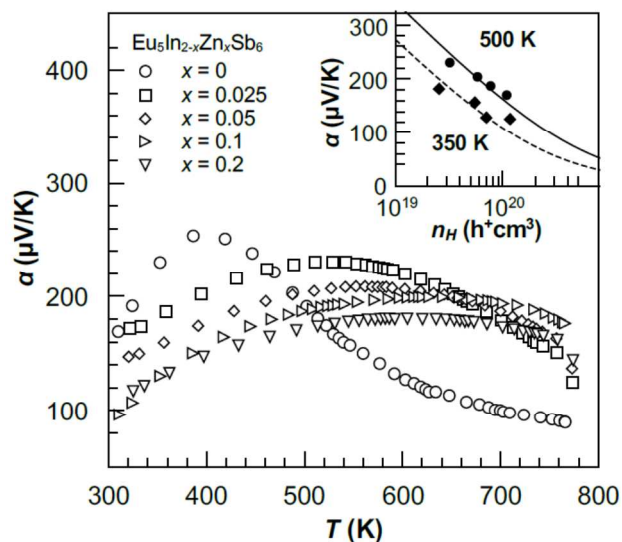
Figure 6: \alpha decreases with increased n_H . A small band gap results in minority carrier activation at lower temperatures. m^* of 1.1 m_e at 350 K and 1.35 m_e at 500 K were used to generate the Pisarenko curves in the inset.
