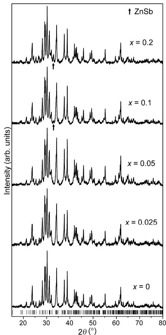
Figure 2: XRD patterns of \text{Eu}_5\text{In}_{2-x}\text{Zn}_x\text{Sb}_6 (Cu- K_{\alpha 1} radiation). Calculated peak positions of \text{Eu}_5\text{In}_2\text{Sb}_6 are indicated by ticks at the bottom [19]. An increasing amount of ZnSb was observed for samples x \geq 0.1 —the most intense peaks are indicated by the arrows.
