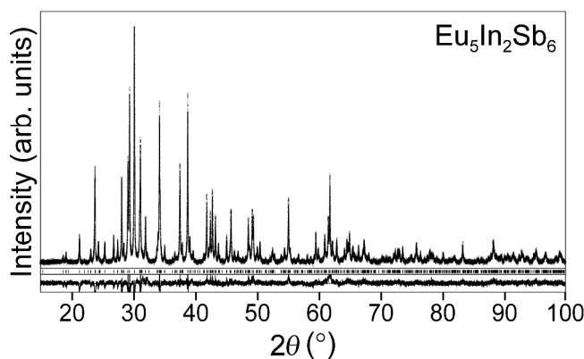
Figure 3: XRD pattern of Eu 5 In 2 Sb 6 (Cu-K α1 radiation). Ticks mark the calculated reflection positions of the target phase while the baseline corresponds to the residuals of a Rietveld refinement based on the reported crystal structure ( R_i = 0.07 , R_p = 0.18 , R_{wp} = 0.15 ) [19].
