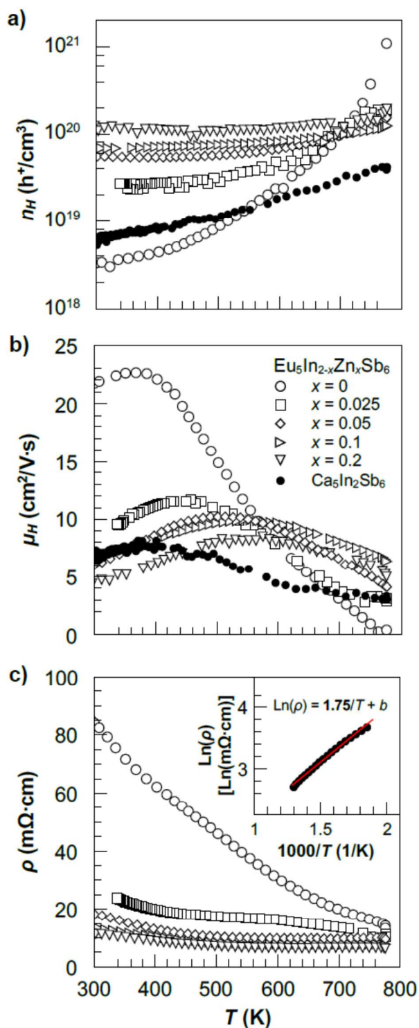
Figure 5: a) The addition of Zn increases n_H , suggesting that Zn is acting as a dopant in \text{Eu}_5\text{In}_2\text{Sb}_6 . b) \mu_H in the undoped sample is higher than in other A_5\text{In}_2\text{Sb}_6 compounds, and appears to be controlled by an activated process below 500 K. c) \rho decreases with increasing dopant concentration. Inset) \rho \propto e^{E_g/2k_B T} yields a band gap of E_g \sim 0.29 eV.
