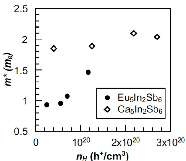
Figure 7: The constant m^* of \text{Ca}_5\text{In}_2\text{Sb}_6 suggests single band behavior while the increasing m^* in \text{Eu}_5\text{In}_2\text{Sb}_6 hints at two band behavior.
