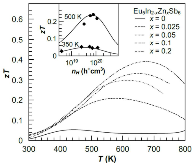
Figure 10: zT plots of \text{Eu}_5\text{In}_{2-x}\text{Zn}_x\text{Sb}_6 ( x = 0, 0.025, 0.05, 0.1, 0.2 ). Inset: the SPB generated curves are in good agreement with the experimental zT values for all samples at 350 K and for x \geq 0.05 at 500 K.
