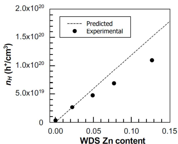
Figure 4: A comparison of the predicted and experimental Hall carrier concentration suggests that the efficiency of Zn doping decreases after a nominal composition of x = 0.05 .
