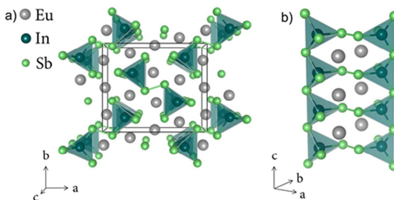
Figure 1: The crystal structure of \text{Eu}_5\text{In}_2\text{Sb}_6 contains 26 atoms per unit cell. a) In (blue) and Sb (green) form covalent bonds while Eu (gray) atoms provide overall charge balance. b) Ladder-like chains formed by corner-linked \text{InSb}_4 tetrahedra along the c direction.
