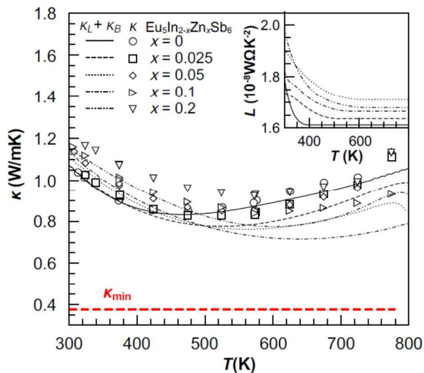
Figure 9: The thermal conductivity of the samples increases as more Zn is added. \kappa_L + \kappa_B are the dominant components in \kappa - \kappa_B has particularly large contributions at higher temperatures. \kappa_{min} is indicated by the red dashed line. The Lorenz factors used to calculate \kappa_e are shown in the inset.
