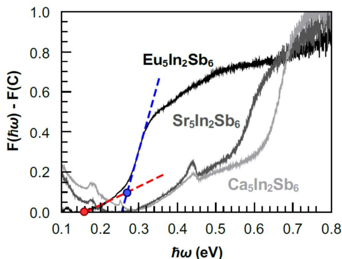
Figure 8: Absorption edge data obtained using DRIFTS for A_5\text{In}_2\text{Sb}_6 ( A = \text{Eu}, \text{Sr}, \text{Ca} ). The red dashed line is the extrapolation to zero which indicates the first transition and the blue indicates the second transition in \text{Eu}_5\text{In}_2\text{Sb}_6 . The extrapolated gap values are indicated by the corresponding large dots. \text{Sr}_5\text{In}_2\text{Sb}_6 and \text{Ca}_5\text{In}_2\text{Sb}_6 have larger transition energies than \text{Eu}_5\text{In}_2\text{Sb}_6 .
