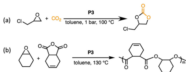
Scheme 2 (a) CO 2 /GC coupling reaction catalysed by crosslinked poly(PPNCl). General reaction conditions: reactions were carried out in a sealed flask on a 12.8 mmol scale of GC and 0.4 mol% crosslinked poly(PPNCl) (mol% as calculated from the number of PPNCl moieties) in 1 mL toluene at 100 °C and 1 bar. (b) Ring-opening polymerisation catalysed by crosslinked poly(PPNCl). General reaction conditions: polymerisation was conducted in toluene at 130 °C. CHO : CDA : PPNCl group = 200 : 100 : 4.
