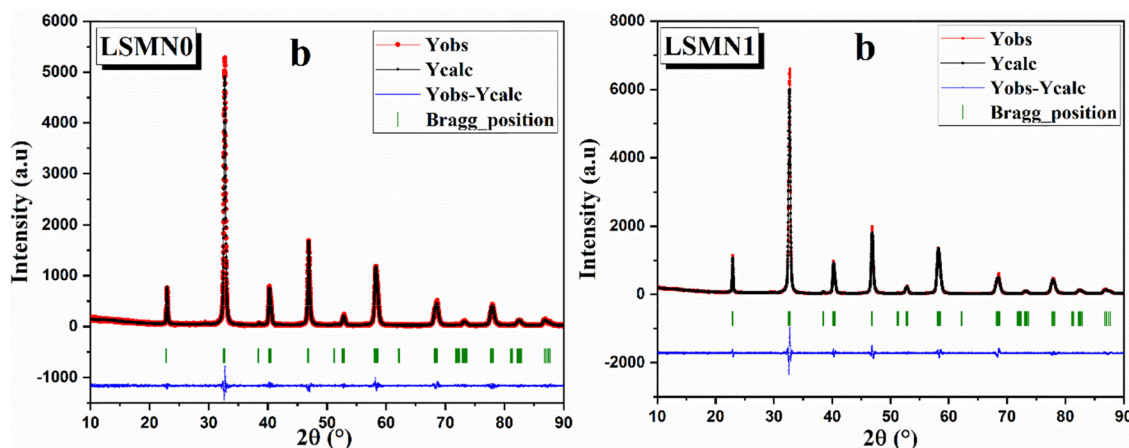
Fig. 1 (a) XRD patterns of LSMN0 and LSMN1 compounds indexed to the rhombohedral R\bar{3}c phase (Ref. Cod: 96-152-1757). The inset shows the most peak shift between the two samples. (b) Rietveld refinement profiles of LSMN0 and LSMN1.
