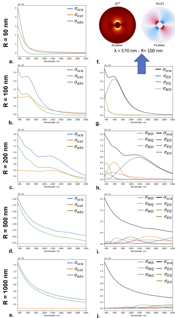
Fig. 6 Calculation of optical cross-sections and field distributions for HEA nanoparticles of different sizes. (a–e) Evolution of scattering ( \sigma_{sca} , blue), absorption ( \sigma_{abs} , green), and extinction ( \sigma_{ext} , orange) cross-sections for nanoparticles with radii of 50, 100, 200, 500, and 1000 nm, showing transitions from Rayleigh to Mie and then to geometrical scattering regimes. (f) Electric field distribution around a 100 nm radius nanoparticle at 570 nm wavelength in the XZ and YZ planes, revealing dipole-like behaviour. (g–j) Multipole decomposition of scattering cross-sections for nanoparticles of increasing size, showing contributions from various electric and magnetic modes (E: electric mode, M: magnetic mode, D: dipole, Q: quadrupole, O: octupole). (k) Temperature elevation of nanoparticles as a function of their radius and the incident wavelength for an incident power of I = 0.1 \mu\text{W} \mu\text{m}^{-2} .
