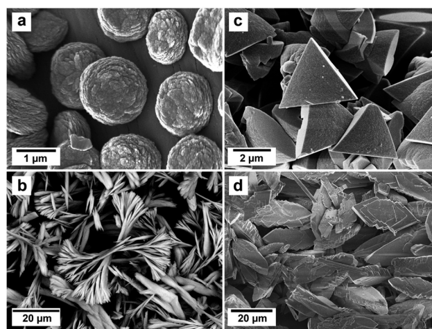
Fig. 2 Spherulitic growth of (a) La-kozoite after La-lanthanite at 21 °C; (b) Pr-kozoite at 35 °C crystallised directly from an amorphous Pr carbonate; (c) La-hydroxylbastnasite formed after La-kozoite via dissolution–recrystallisation; (d) Dy-kozoite formed after Dy-tengerite via dissolution–recrystallisation.
