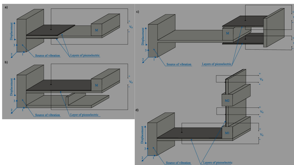
Fig. 17 Various alternative cantilever beams as the structure base of a piezoelectric generator. Reproduced with permission. 428 Copyright 2013, Pomary Automatyka Robotyka.
