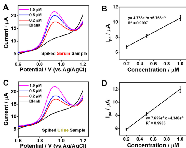
Fig. 7 DPV curves of NiMn 2 O 4 /CNT-GCE obtained for (A) spiked human serum and (C) spiked urine samples with increasing MTX concentrations in 0.1 M PBS (pH 7.0). (B) and (D) show the corresponding linear plots between I_{pa} and MTX concentrations for the serum and urine samples, respectively.
