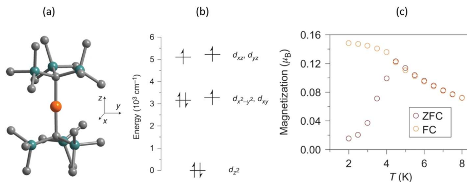
Fig. 2 Structure of [\text{FeC}(\text{SiMe}_3)_2]^{1-} from the crystal structure of [\text{K}(\text{crypt-222})][\text{FeC}(\text{SiMe}_3)_2] . Orange, turquoise and grey spheres represent Fe, Si and C, respectively (a). Energies of 3d molecular orbitals from ab initio ligand field CASSCF(NEVPT2) calculations (b). Low-temperature magnetisation data reveal blocking at 4.5 K, with divergence between field-cooled (FC) and zero-field-cooled (ZFC) measurements (c) (adapted from ref. 1 with permission of Nature Publishing Group, copyright 2013).
