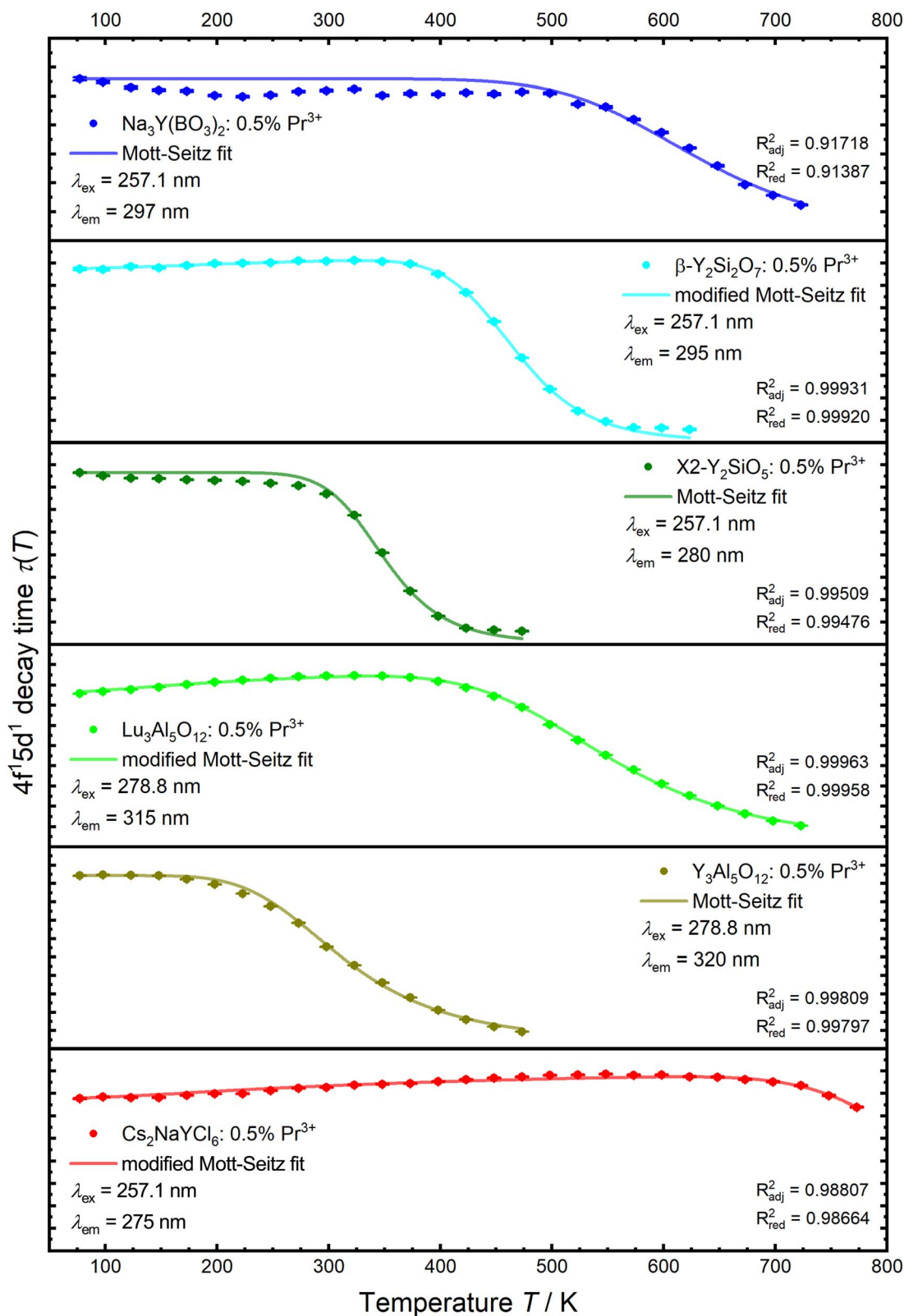
Fig. 6 Luminescence decay times of 4f^{15}d^1 configuration states of \text{Pr}^{3+} in the synthesized host compounds as a function of temperature with a fit to a Mott-Seitz law (eqn (1) or (3)). Decay times were derived from the exponential fit using eqn (S1).†
