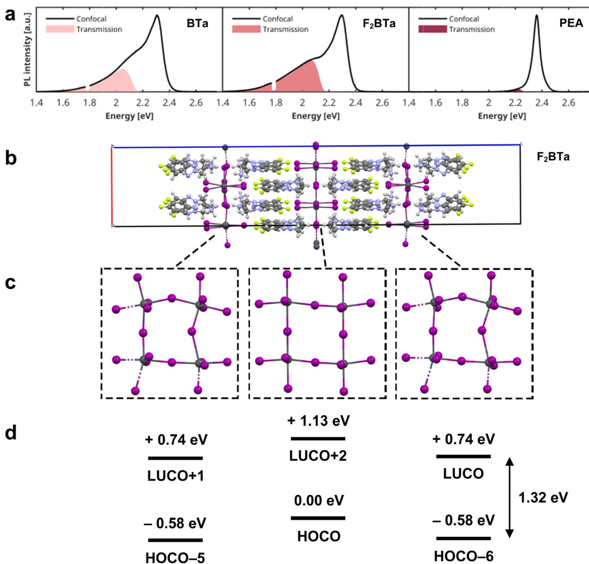
Fig. 3 (a) Single-crystal PL spectra of (\text{BTa})_2\text{PbI}_4 , (\text{F}_2\text{BTa})_2\text{PbI}_4 , and (\text{PEA})_2\text{PbI}_4 at room temperature after excitation at 3.06 eV (405 nm), comparing the PL spectra collected using two different measurement geometries: confocal (solid line) and transmission geometry (shaded area); see the main text for details. At 1.79 eV, a narrow artifact due to a luminescent impurity in the cryostat window has been removed from all spectra. (b) Optimized structure of the (\text{F}_2\text{BTa})_2\text{PbI}_4 theoretical surface model. (c) Enlarged images of the inorganic framework at surface and bulk positions to illustrate structural distortion. (d) Diagram of the lowest-energy HOCO/LUCO transitions involving only the surface and bulk inorganic groups, respectively.
