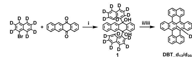
Scheme 1 Synthetic route to DBT_d 12 and DBT_d 20 . Reagents and conditions: (i) n -BuLi, 5,12-naphthacenequinone, THF, -78^\circ\text{C} , 60%; (ii) \text{AlCl}_3 , NaCl, 140^\circ\text{C} , 10 min, 20% for DBT_d 12 ; (iii) \text{AlCl}_3 , chlorobenzene-d 5 , 100^\circ\text{C} , 1 h, 50% for DBT_d 20 .
