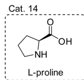
Scheme 34 Synthesis of iodopyrrole-3-carboxaldehydes catalyzed by Cat. 14.
