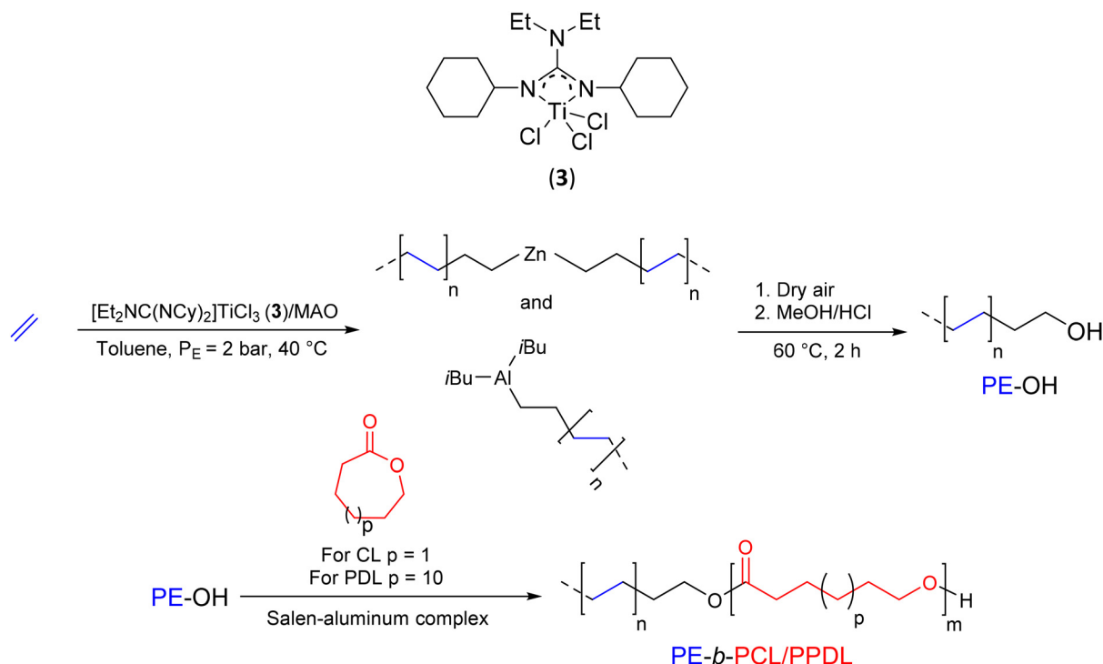
Scheme 4 Synthesis of PE-OH and PE- b -PCL/PPDL diblock copolymers by the combination of CTP and ROP. 2
