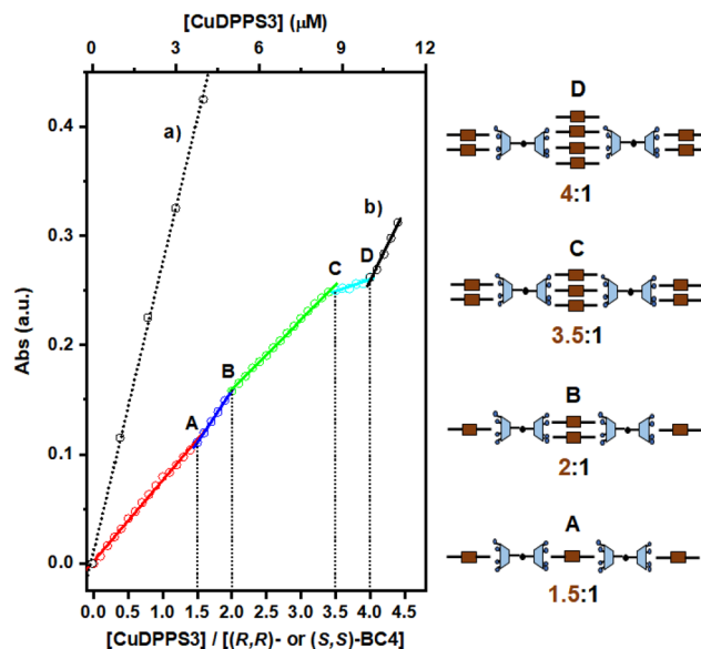
Fig. 6 Variation in the absorbance of the \text{CuDPPS3} Soret band ( \lambda = 405.5\text{ nm} ) observed upon: (i) increase of the porphyrin concentration in water at \text{pH} = 2.0 (dotted black trace labelled as (a)); (ii) portion-wise addition ( 0.25\text{ }\mu\text{M} ) of \text{CuDPPS3} to a 2.5\text{ }\mu\text{M} aqueous solution of (R,R) - or (S,S) - \text{BC}_4 at \text{pH} = 2.0 (multi-coloured trace labelled as (b)). The break-points are labelled as A, B, C, and D. The cartoons sketched on the right hand-side represent the likely structures of the complexes A, B and C, formed at the corresponding break-points .
