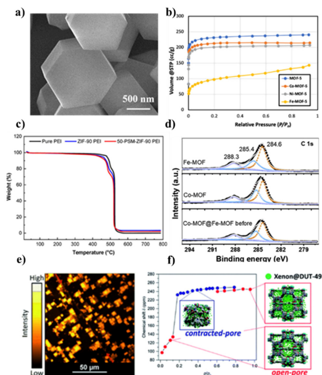
Fig. 2 Main MOF characterization techniques: (a) SEM images of ZIF-8 (reproduced from ref. 89 © 1996–2024 MDPI); (b) nitrogen adsorption isotherms at -196^\circ\text{C} of MOF-5 and doped MOF-5 (reproduced from ref. 90 © 1996–2024 MDPI); (c) TGA of pure PEI, ZIF-90 PEI and 50-PSM-ZIF-90 PEI membranes (reproduced from ref. 91 © 1996–2024 MDPI); (d) XPS spectra of Fe-MOF, Co-MOF, Co-MOF@Fe-MOF, and the hybrid MOF (reprinted with permission from ref. 92; Copyright © 2024 with permission from Elsevier. Also Lancet special credit, reprinted from The Lancet from ref. 92; Copyright © 2024 with permission from Elsevier); (e) confocal fluorescence imaging of defects in a MOF-5 single-crystal (reproduced from ref. 93 © 1999–2024 John Wiley & Sons, Inc. or related companies); (f) chemical shift of xenon adsorbed in DUT-49 at -73^\circ\text{C} measured during the adsorption experiment (red symbols indicate DUT-49op signals; blue symbols indicate DUT-49cp signals) (reprinted with permission from ref. 94; Copyright(2017) American Chemical Society).
