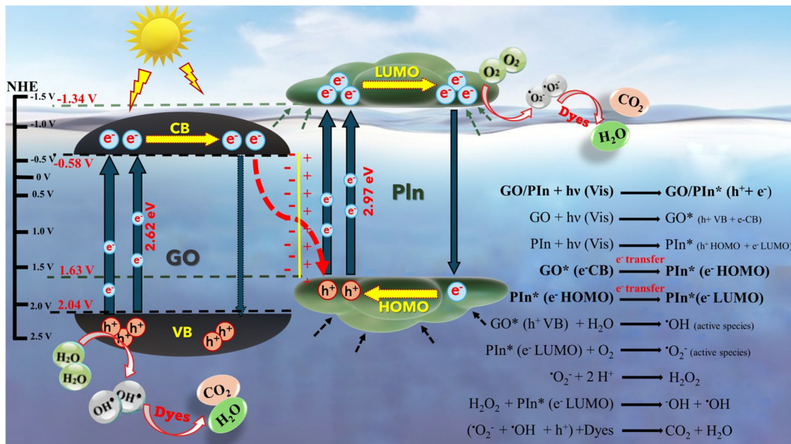
Fig. 13 Plausible photocatalytic mechanism of dye degradation by the GO/PIn composite: diagrammatic representation and proposed pathway scheme.
