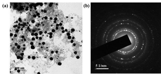
Fig. 5 (a) TEM images of the AIGO composite depicting the presence of Au and Ga 2 O 3 . (b) SAED diffraction pattern of AIGO with ring patterns and bright spots confirming the crystallinity of the composite. Reproduced with permission from ref. 28 and 30.
