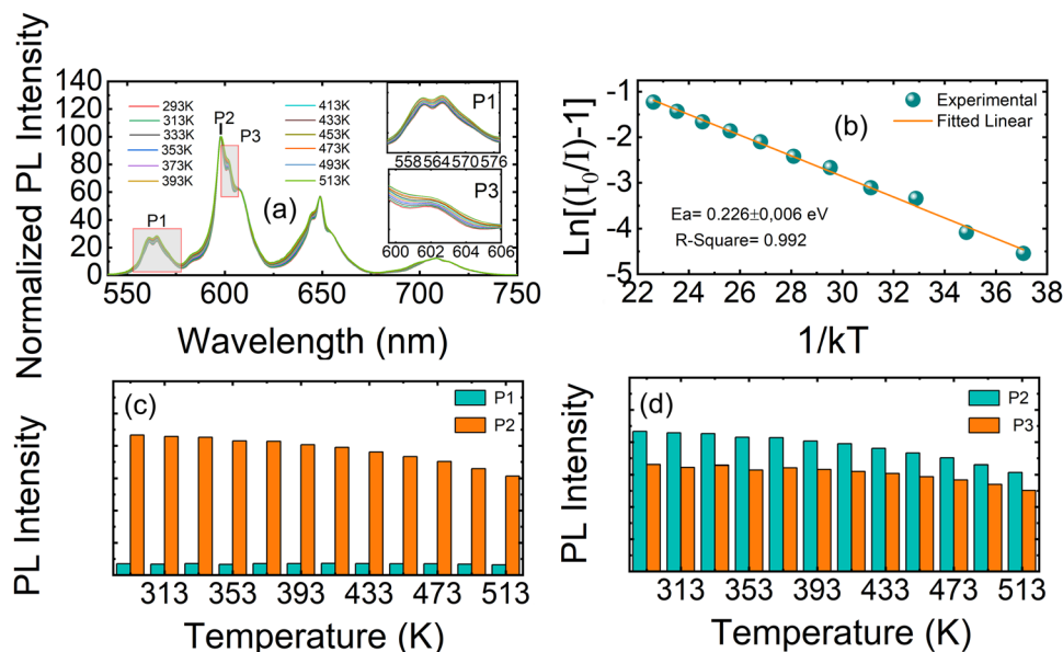
Fig. 10 (a) Emission spectra as a function of temperature (293–513 K) of \text{Ca}_3\text{La}_7(\text{SiO}_4)_5(\text{PO}_4)_2\text{:}6\text{ at}\% \text{Sm}^{3+} under 404 nm excitation; (b) plot of \ln[(I_0/I) - 1] versus activation energy 1/kT for thermal quenching of \text{Ca}_3\text{La}_7(\text{SiO}_4)_5(\text{PO}_4)_2\text{:}6\text{ at}\% \text{Sm}^{3+} for the 598 nm ( {}^4\text{G}_{5/2} \rightarrow {}^6\text{H}_{7/2} ) transition; the bar graph shows the evolution of (c) P1 and P2 , (d) P2 and P3 for \text{Ca}_3\text{La}_7(\text{SiO}_4)_5(\text{PO}_4)_2 doped with 6% \text{Sm}^{3+} as a function of temperature.
