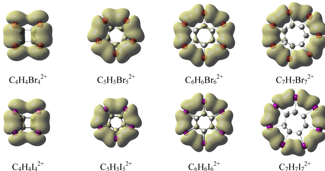
Fig. 8 Top view of the \sigma -EDDB H function isosurfaces (isovalence: 0.001 a.u.) for dicationic halogenated cycloalkanes.
