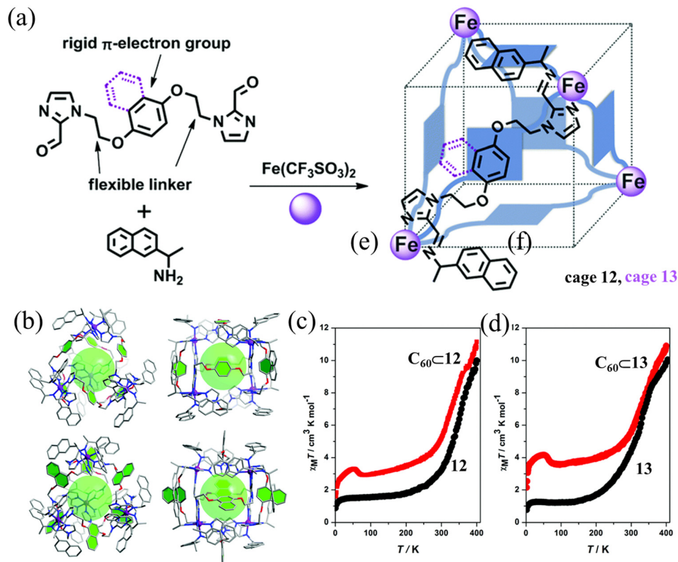
Fig. 12 (a) Synthesis method of cages 12 and 13 . (b) Crystal structures of 12 (top) and 13 (bottom). \chi_{\text{m}}T vs. T plots for 12 and \text{C}_{60}<\mathbf{12} (c) and 13 and \text{C}_{60}<\mathbf{13} (d). 83
