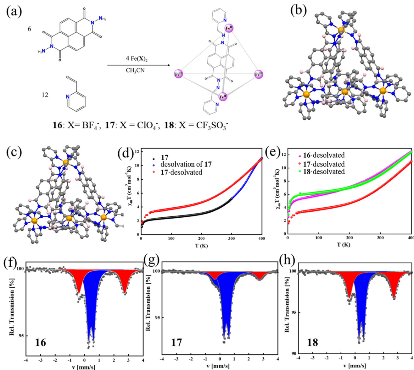
Fig. 16 (a) Synthesis method of cages 16 – 18 . Crystal structures of 17 (b) and 18 (c). (d) \chi_m T vs. T plots for 17 (black circles), desolvation of 17 (blue circles) and 17 -desolvated (red circles). (e) \chi_m T vs. T plots for desolvated 16 – 18 . ^{57}\text{Fe} Mössbauer spectra of desolvated 16 (f), 17 (g) and 18 (h) recorded at 80 K. 86
