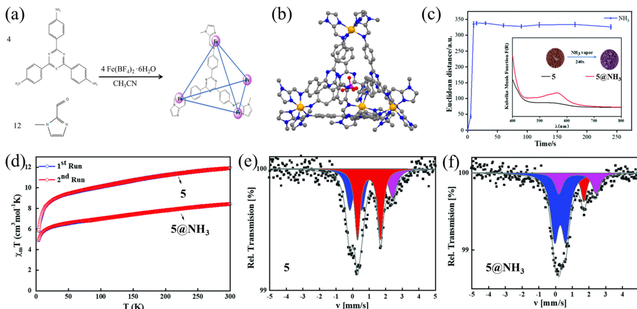
Fig. 7 Synthesis method (a) and crystal structure (b) of 5. (c) Response time of 5 to \text{NH}_3(\text{g}) at room temperature. Inset: diffuse reflectance spectroscopy and photos of 5 and 5@ \text{NH}_3 . \chi_m T vs. T plots (d) and ^{57}\text{Fe} Mössbauer spectra for 5 (e) and 5@ \text{NH}_3 (f). 53
