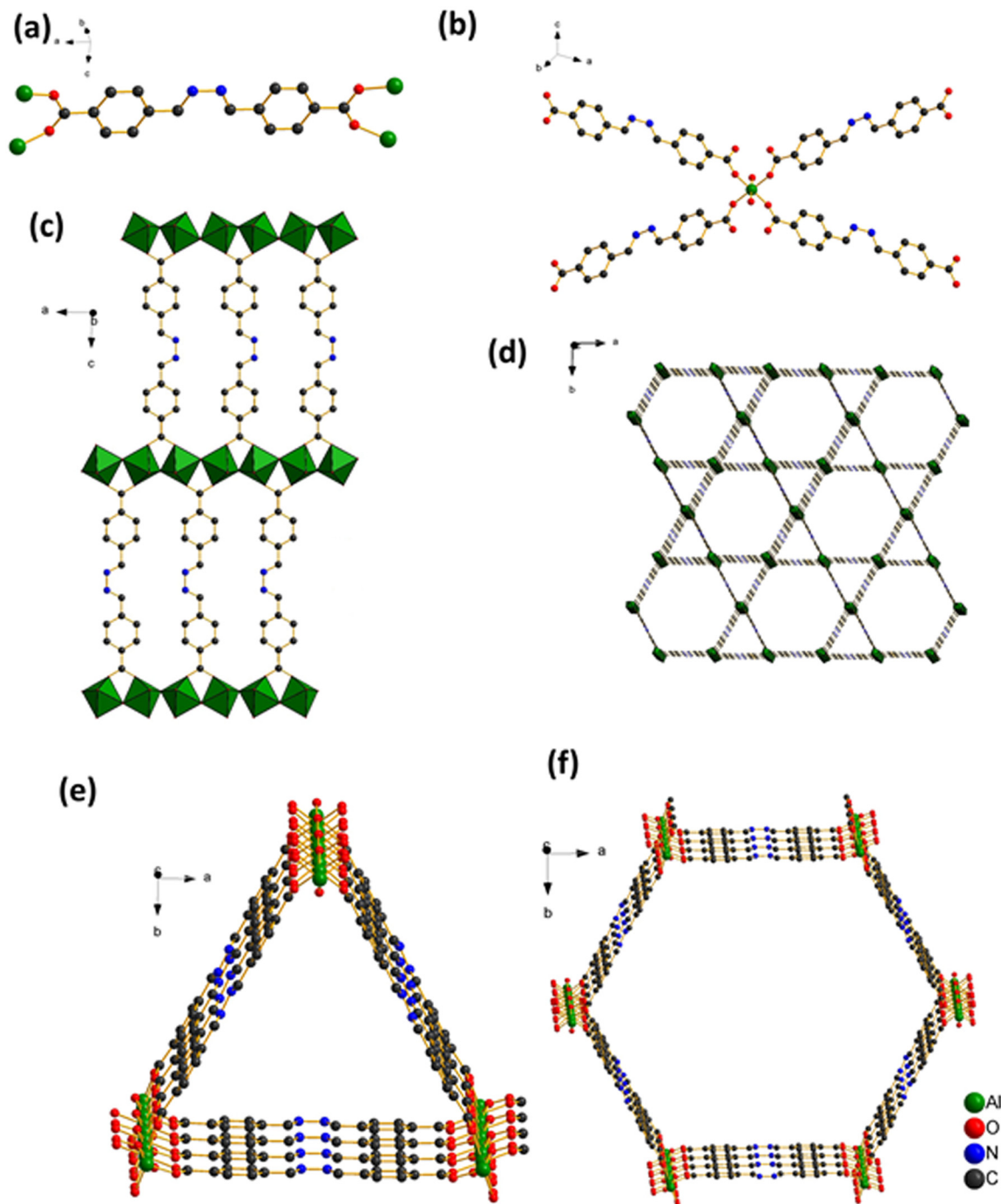
Fig. 1 (a) The coordination environment of the H 2 DMDA ligand in the AlDMDA-68. (b) The aluminum ion in AlDMDA-68 is coordinated in an octahedral arrangement. (c) Coordination modes of one-dimensional inorganic chains and their ligands. (d) A 3D structure of AlDMDA-68. (e) Microporous triangular window channels of AlDMDA-68. (f) Mesoporous hexagonal window channels of AlDMDA-68.
