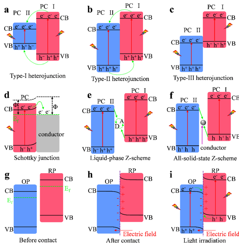
Fig. 2 Schematic diagram of different types of heterojunction photocatalysts. (a) Type I, (b) type II, (c) type III, (d) Schottky heterojunction, (e) liquid-phase Z-scheme, (f) all-solid-state Z-scheme, and S-Scheme, (g) before contact, (h) after contact, and (i) light irradiation photocatalytic systems. The labels D and A denote the electron donor and acceptor in (e), respectively.
