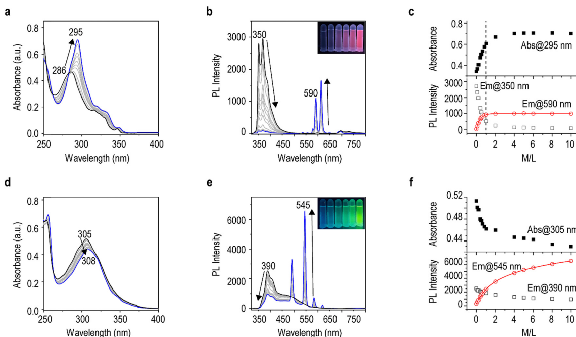
Fig. 3 Ratiometric detection analyses. (a) and (d) Absorption and (b) and (e) emission spectra changes with the addition of \text{Eu}(\text{III})/\text{Tb}(\text{III}) into 2 \times 10^{-5} M Phen-2DIBA / Phen-2DIBA-re in water. The evolutions of absorption (up) and emission (bottom) at characteristic wavelengths as functions of M/L ratios for (c) Phen-2DIBA and (f) Phen-2DIBA-re . The red curves show the nonlinear fitting to the data (ExpGro 1 in panel (c) and ExpGro 3 in panel (f)). The arrows in all figures are used to show changes during the titrations.
