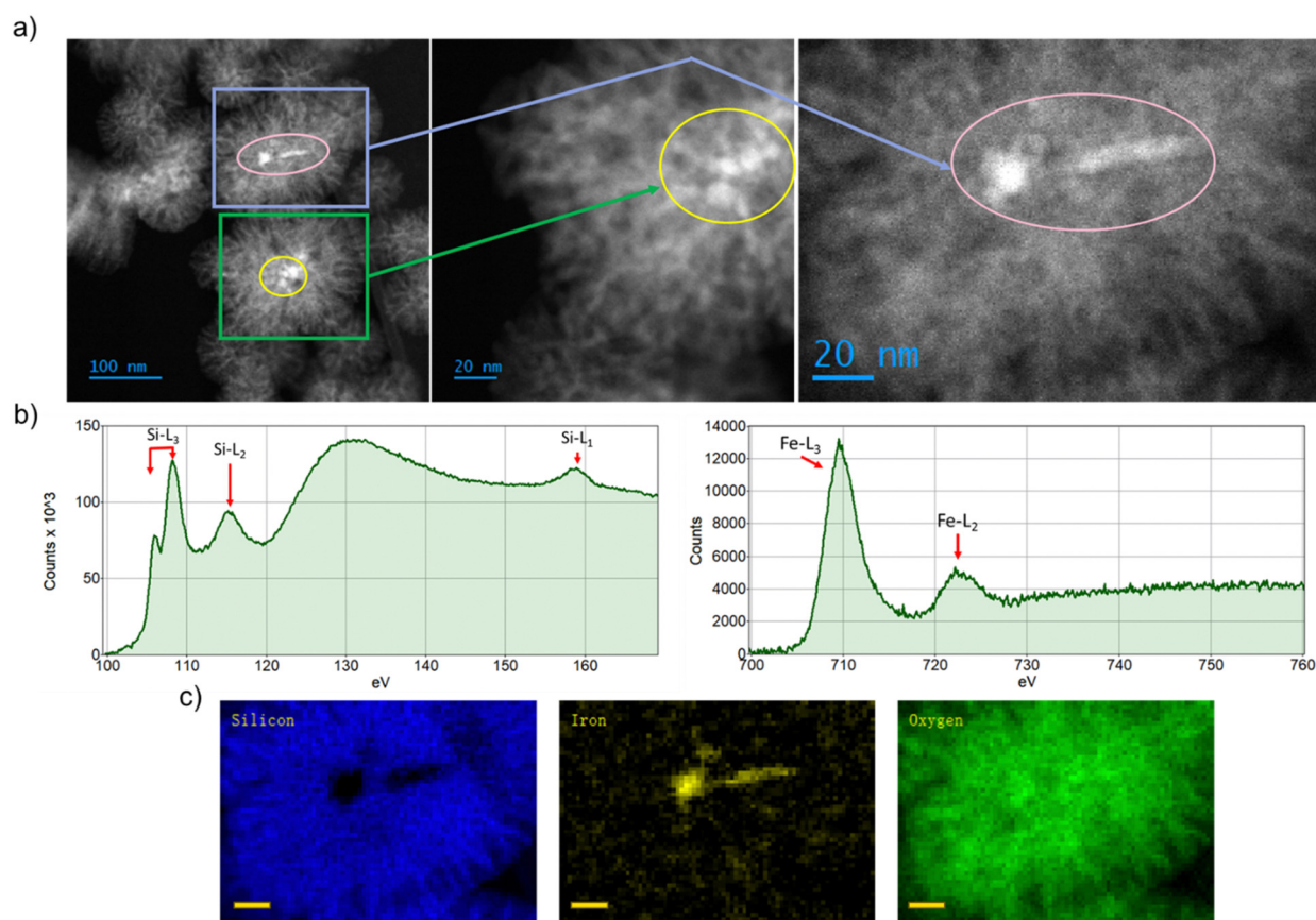
Fig. 1 FeSiNP characterisation – (a) ADF-STEM images showing iron oxide in the central region and porous silica dendritic structure outside, (b) Si L- and Fe L-edges EELS spectra confirming the oxidation states of Si and Fe as silica and iron oxide, and (c) STEM-EELS maps of silicon, iron and oxygen showing the localisation of different elements in the core and shell of synthesised FeSiNPs (scale bar = 20 nm).
