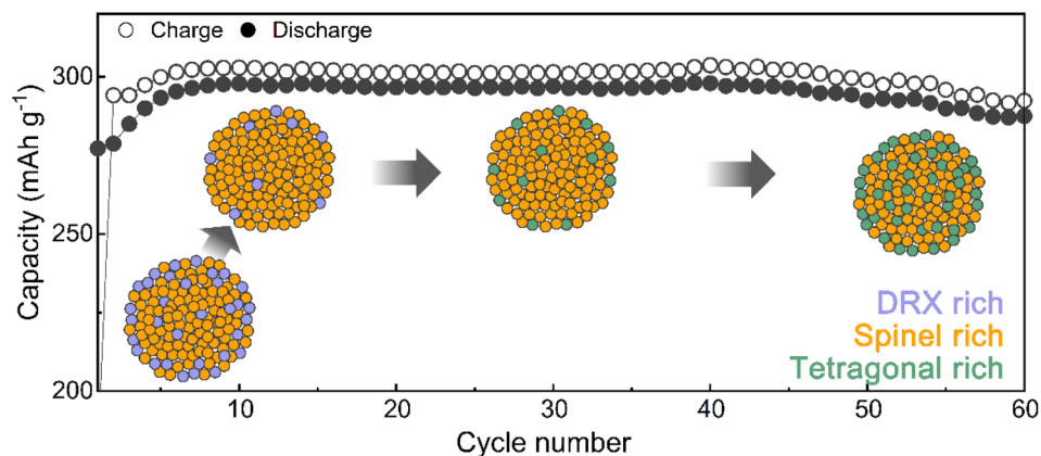
Fig. 5 Phase evolution mechanism in \text{Li}_{1.33}\text{Mn}_2\text{O}_4 with DRX-rich surface mitigating voltage decay and capacity degradation during electrochemical cycling.
