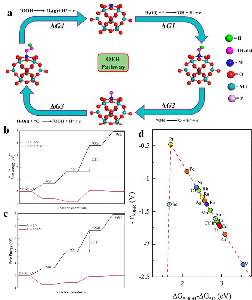
Fig. 5 (a) Schematic of the 4e⁻ OER pathway of the 4H site via the M₁/PMA cluster, reproduced with permission. 21 Copyright 2021, American Chemical Society. (b) Free energy diagrams of basic steps of the Pd@Sb monolayer and (c) Pd@Sb monolayer at different potentials. (d) The volcano curve between negative OER overpotential and \Delta G_{\text{OOH}^*} - \Delta G_{\text{O}^*} for TM@Sb monolayers. Reproduced with permission. 54 Copyright 2021, Royal Society of Chemistry.
