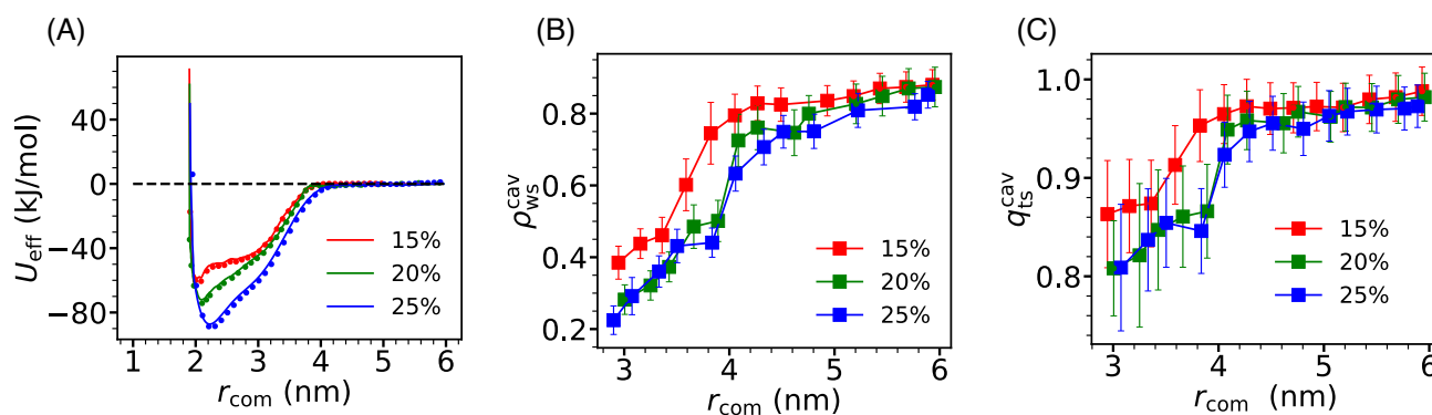
Fig. 8 (A) The potential of mean force ( U_{\text{eff}} ) of the PE-grafted Si-NPs in water in water at T = 300 K and P = 1 bar for three different surface ligand (PE) coverages — 15%, 20%, and 25%. We note the gradual increase of the depth of the PMF on increasing the surface grafting density. (B) The scaled average density ( \rho_{\text{ws}}^{\text{cav}} ) of the confined water as a function of the inter-particle center-of-mass separation ( r_{\text{com}} ) for PE-grafted Si-NPs. (C) The same is shown for the scaled tetrahedral order parameter q_{\text{ts}}^{\text{cav}} .
