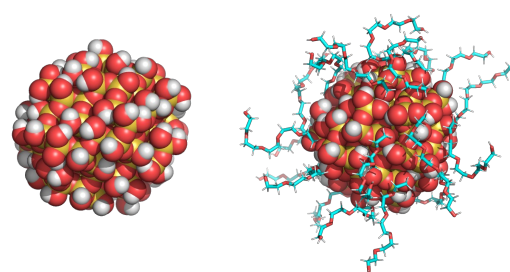
Fig. 1 A snapshot of the bare and polymer-grafted silica nanoparticle is shown. The grafting polymer chain length is 5 (monomer units) and the grafting (surface) density is 1.75 chains/nm 2 for all the polymer types (PEG, PE, and PMMA) studied in this work.
