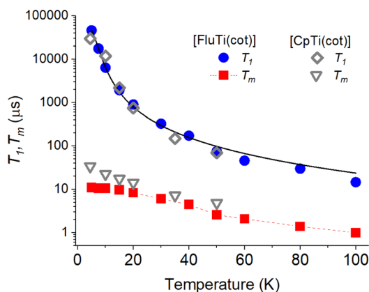
Fig. 4 Temperature dependence of the T_1 and T_m of a 0.5 mmol L -1 solution of [FluTi(cot)] in toluene-d 8 , superimposed to those of [CpTi(cot)] we reported in ref. 5. The black solid line corresponds to the computed ( T_1 ) values (see text).
