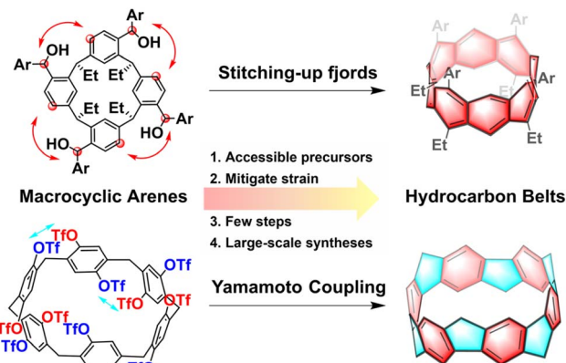
Fig. 1 Strategies and advantages for the synthesis of hydrocarbon belts using traditional macrocyclic arenes.
