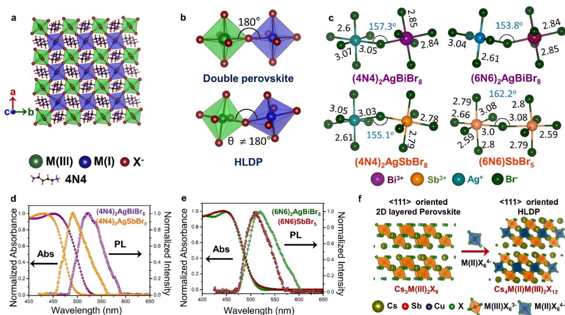
Fig. 5 Schematic representation of (a) the octahedra with M(I) and M(III) centers in the inorganic layer of double perovskite, and (b) the corresponding octahedral tilting. (c) Variations of bond length (in Å) and bond angle (in degrees) in (4N4)_2AgBiBr_8 , (4N4)_2AgSbBr_8 , (6N6)_2AgBiBr_8 , and (6N6)SbBr_5 . 11 Optical absorption, and PL spectra of (d) (4N4)_2AgBiBr_8 , and (4N4)_2AgSbBr_8 , and (e) (6N6)_2AgBiBr_8 , and (6N6)SbBr_5 . 11 (f) Schematic for the formation of LDPs from single layered <111> oriented perovskites. Reproduced with permission from ref. 11, copyright (2023) Royal Society of Chemistry.
