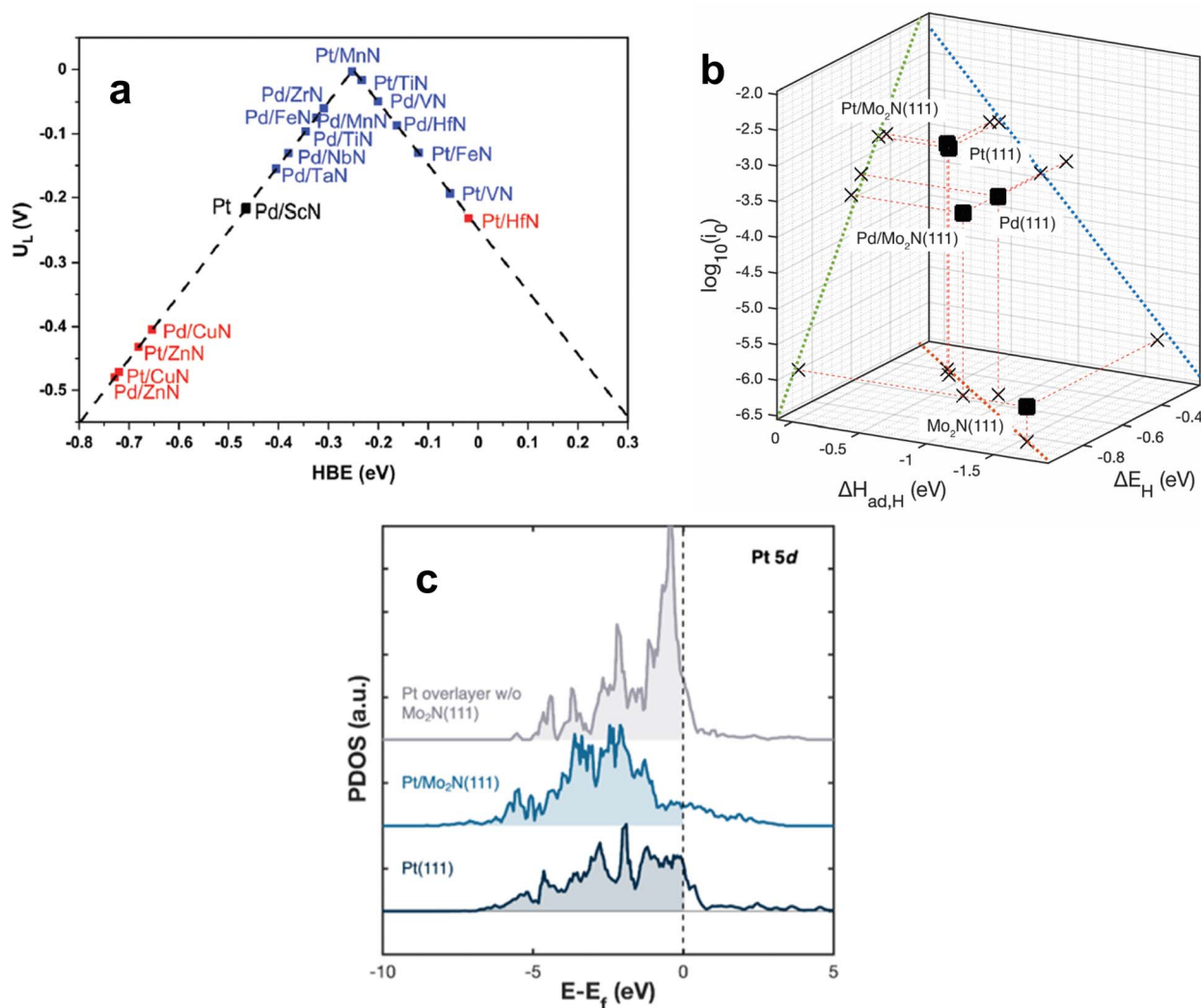
Fig. 7 (a) Volcano relationship for Pt-modified TMNs. (b) Correlation between the HER activity ( \log_{10}(j_0) ) and the binding strength of atomic hydrogen determined by TPD ( \Delta H_{\text{ad,H}} ) and DFT ( \Delta E_{\text{H}} ). (c) Projected density of states (PDOS) for Pt and Pt/TMN surfaces. (a) Reprinted from ref. 114 with permission from the Royal Society of Chemistry, Copyright 2022. (b and c) Reprinted from ref. 37 with permission from the American Chemical Society, Copyright 2023.
