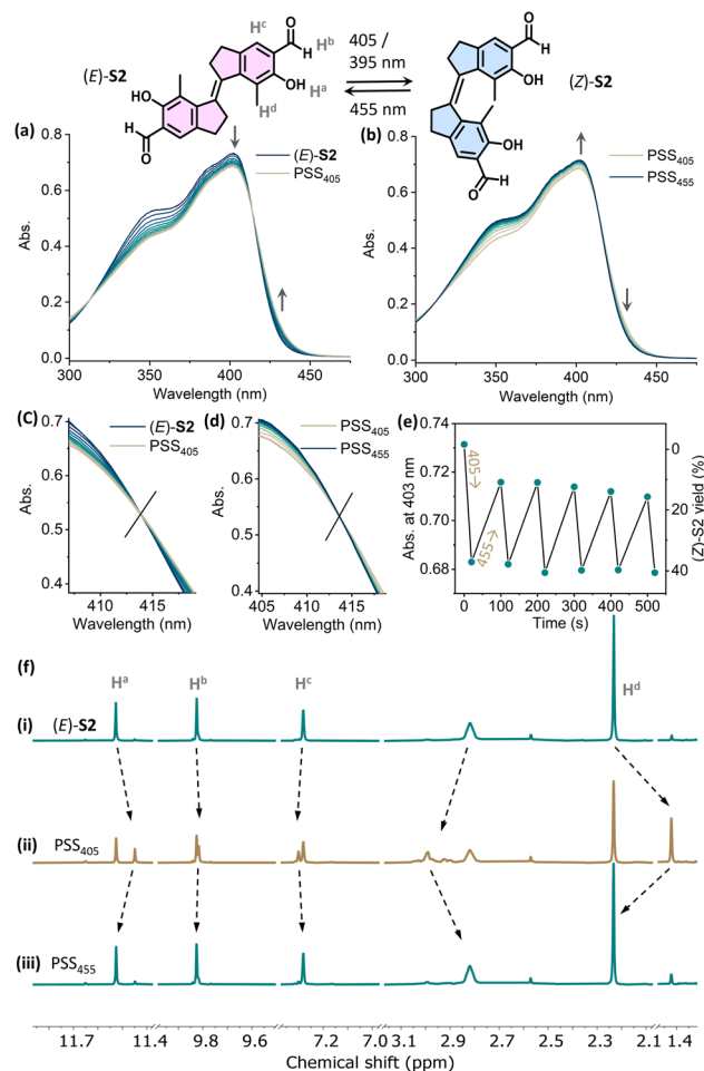
Fig. 4 Changes in the UV-vis absorption spectra starting from (a) ( E )-S2 (24 μM in CH 2 Cl 2 , 298 K) upon irradiation with 405 nm light to PSS 405 and (b) upon subsequent irradiating with 455 nm light to PSS 455 . Enlarged spectra at the isosbestic point of (c) E to Z isomerization and (d) Z to E back-switching. (e) Plots of the absorption at λ = 403 nm upon sequential irradiation with 405 nm and 455 nm light. (f) Changes in 1 H NMR spectra of (i) ( E )-S2 (2.9 mM in CD 2 Cl 2 , 298 K, 500 MHz), (ii) upon irradiation with 405 nm light to PSS 405 , and (iii) upon subsequent irradiation with 455 nm light to PSS 455 .
