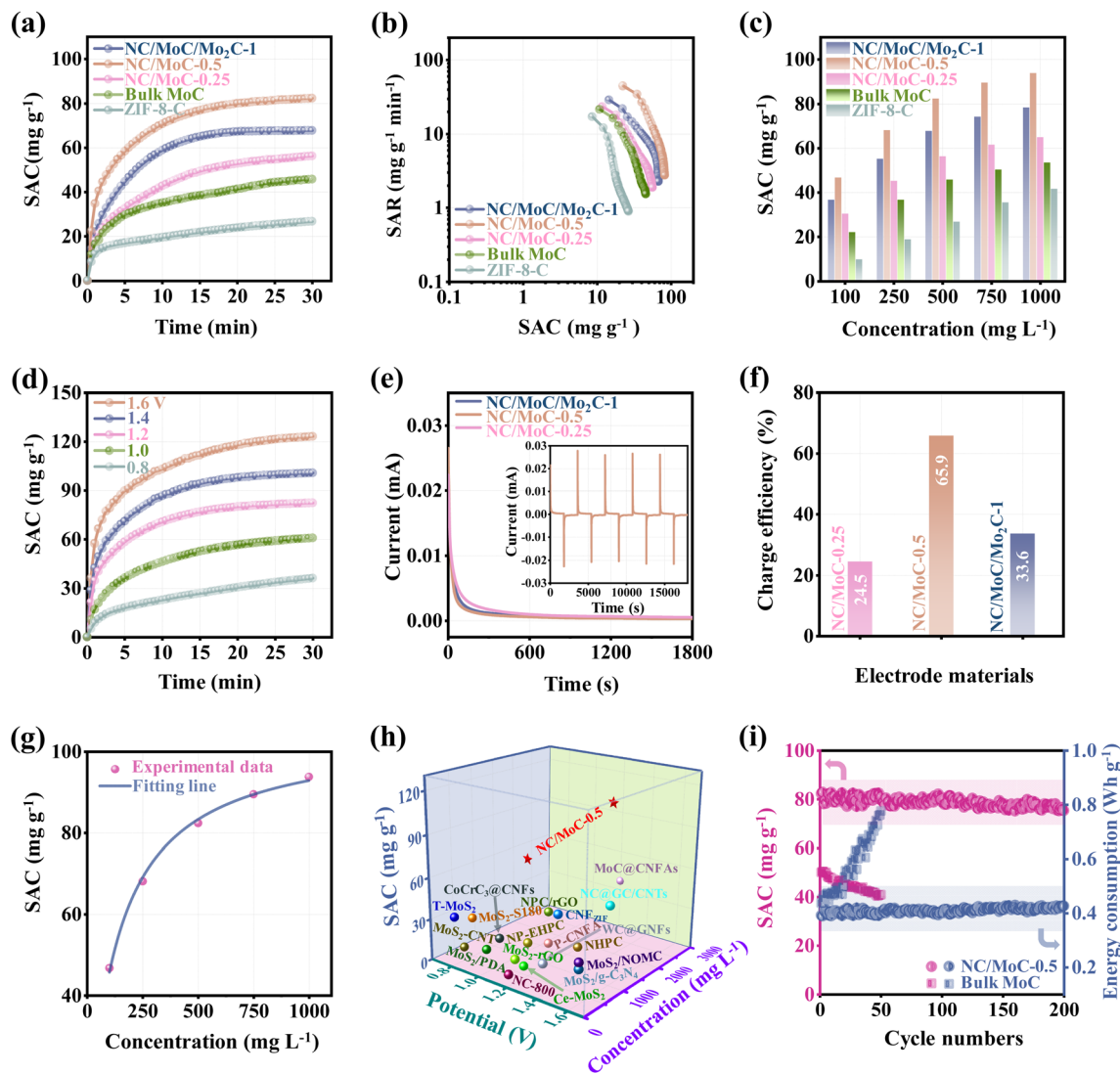
Fig. 4 (a) Dynamic SAC versus deionization time plots, and (b) corresponding CDI Ragone plots of the three NC/Mo 2 C-x, bulk MoC, and ZIF-8-C in 500 \text{mg L}^{-1} NaCl solution at 1.2 V. (c) SAC values at different NaCl concentrations from 100 to 1000 \text{mg L}^{-1} for the three NC/Mo 2 C-x, bulk MoC, and ZIF-8-C (applied voltage: 1.2 V). (d) Dynamic SAC versus deionization time plots of NC/MoC-0.5 with an initial concentration of 500 \text{mg L}^{-1} using different voltages from 0.8 to 1.6 V. (e) Current response curves of the three NC/Mo 2 C-x, and the corresponding current variation of NC/MoC-0.5 during the desalination/regeneration cycle (inset). (f) The calculated charge efficiencies of the three NC/Mo 2 C-x. (g) The fitted isotherm adsorption curves of the Langmuir model (applied voltage: 1.2 V; NaCl concentration: from 100 to 1000 \text{mg L}^{-1} ). (h) Comparison of CDI performance between NC/MoC-0.5 and some reported transition metal carbides/dichalcogenides or MOF-derived carbons. (i) The recycling performance of bulk MoC and NC/MoC-0.5, along with their corresponding energy consumption changes over 200 cycles (applied voltage: 1.2 V; NaCl concentration: 500 \text{mg L}^{-1} ).
