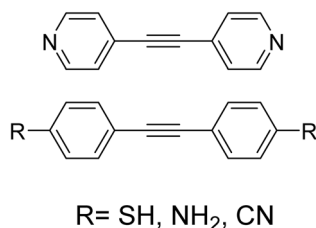
Fig. 40 The tolane compounds used for investigation of JFP. 47
