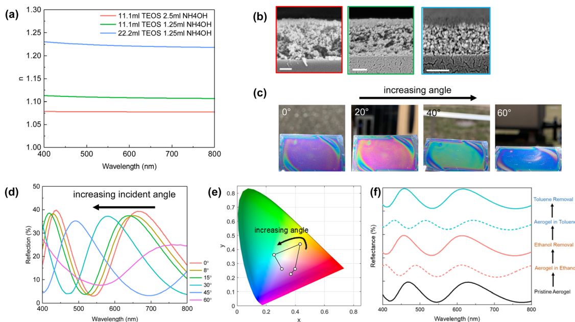
Fig. 27 (a) Spin-coated aerogels with different refractive indexes by changing TEOS concentration. (b) Cross-section SEM image of aerogels with a refractive index of 1.07, 1.14 and 1.23 (from left to right). (c) Photos, (d) angle-resolved reflection spectra, and (e) corresponding CIE diagram of 15 nm Al/Aerogel ( n = 1.07 )/Si film at various angles showing a large color change. (f) Reflection spectra of 15 nm Al/Aerogel ( n = 1.07 )/Si immersed in solvents ( i.e. ethanol and toluene) and upon solvent removal.
