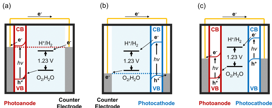
Fig. 2 Energy diagrams of solar water-splitting PEC cells for (a) photoanode, (b) photocathode, and (c) combined photoanode and photocathode configurations.
