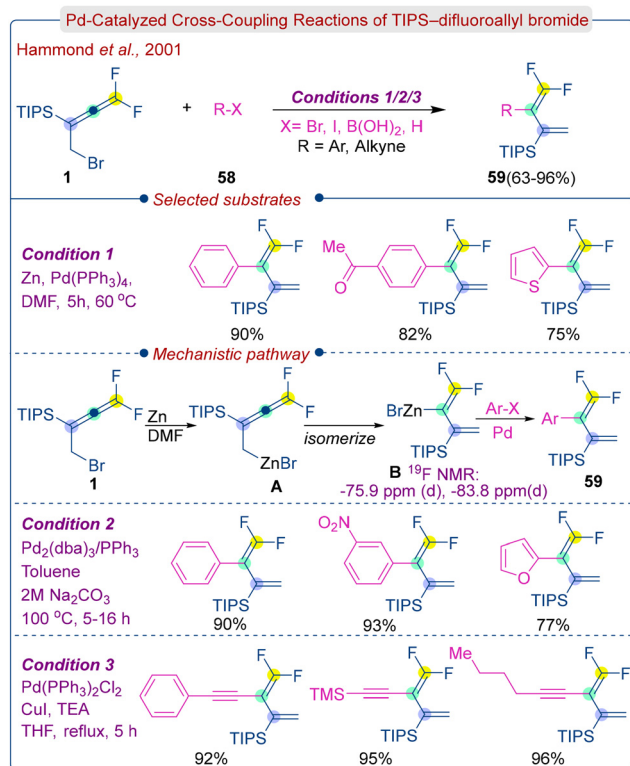
Scheme 26 Pd-Catalyzed cross-coupling reactions of TIPS–difluoroalkyl bromides.
