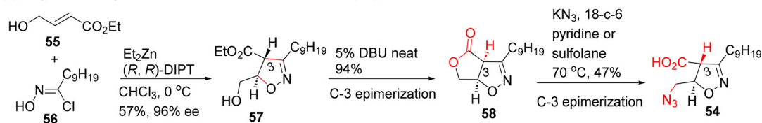
(b) Asymmetric synthesis of trans-azidoisooxazoline ( 54 )
