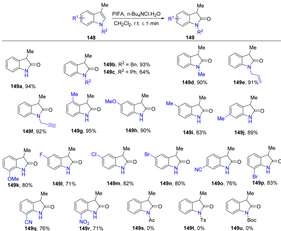
Scheme 61 Synthesis of substituted indole derivatives 148 .
