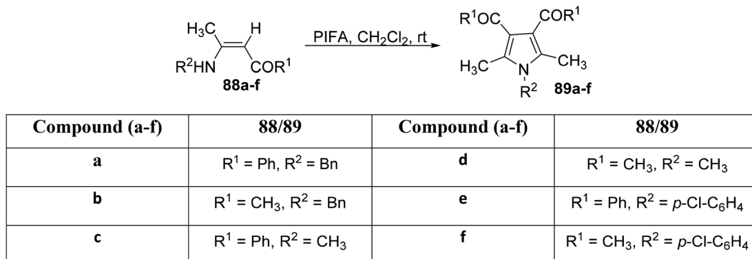
Scheme 32 Synthesis of substituted pyrroles 89a–f .
