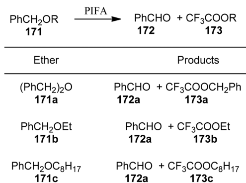
Scheme 71 Oxidation of benzyl ethers 171 .
